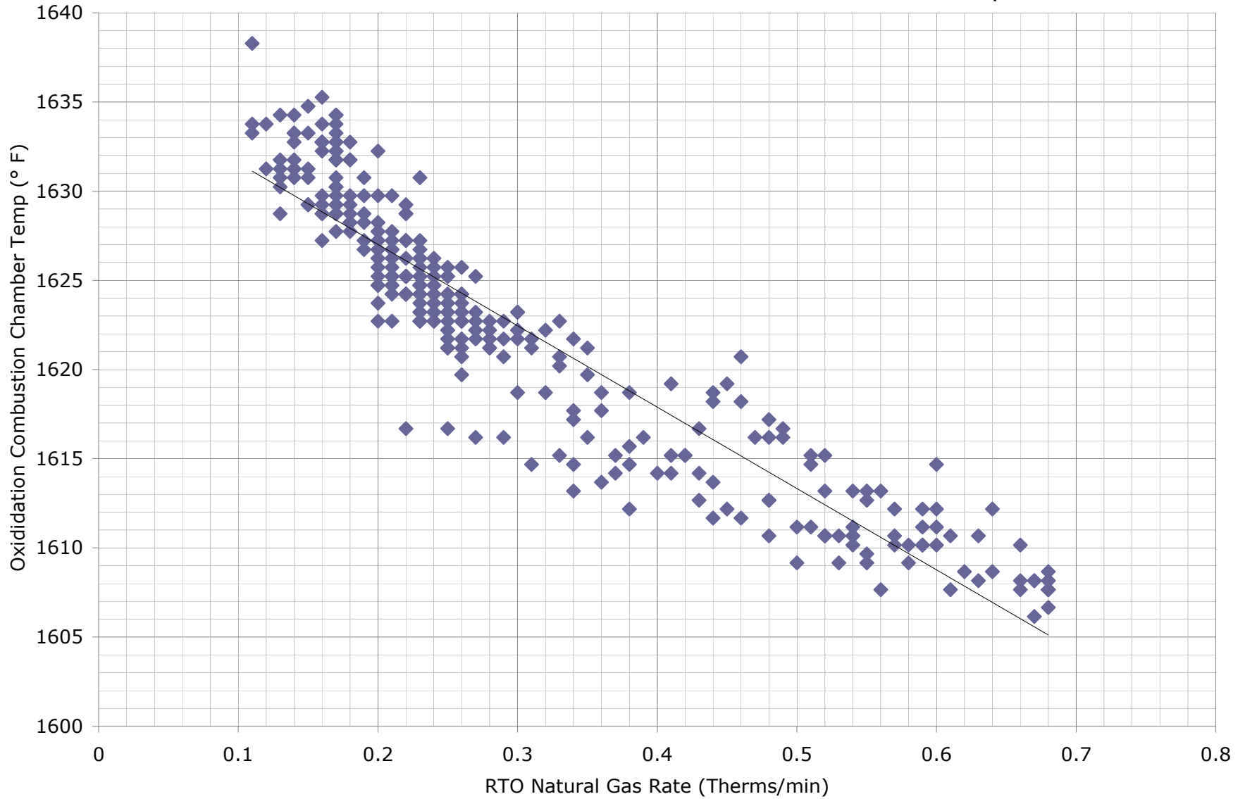
RTO Natural Gas Rate vs Oxidation Combustion Chamber Temperature
